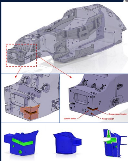
▼ Location of front suspension inserts in chassis & detailed design
