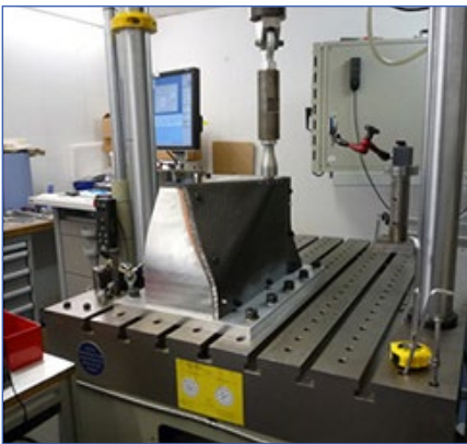
Section of chassis with insert being tested to validate performance
