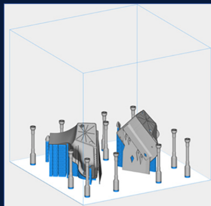
▲ Chassis insert build setup
