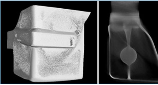
CT scan of printed chassis inserts
