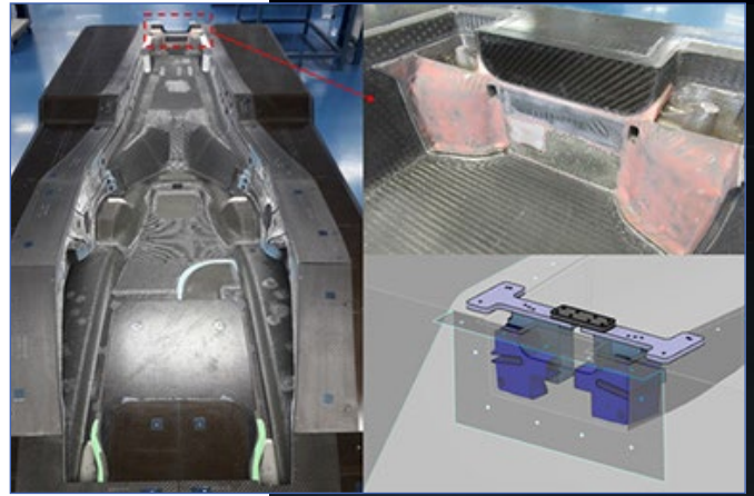
Chassis lower half with inserts bonded in place before laminating of inner skin
